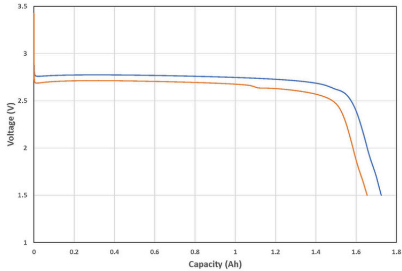
Contego P1400 5 mA and 20 mA Discharge at 37°C
