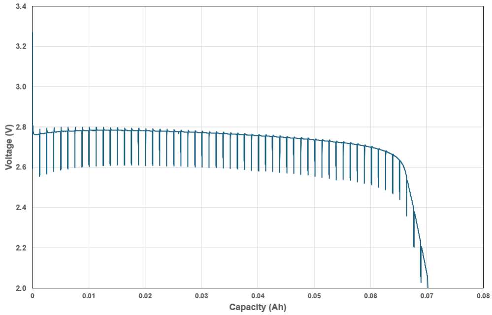
P65 37°C 4-Week Capacity Discharge 1 mA Pulse for 180 Seconds every 12 Hours 100 \mu A Baseline, 70 mAh
