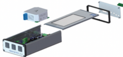
Exploded view of the Development kit with its internal module
